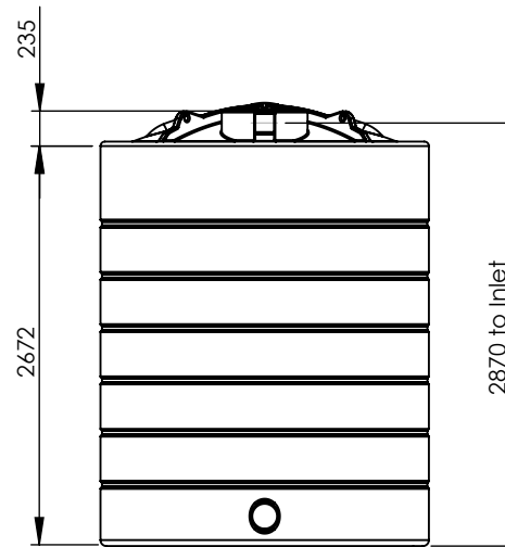
Side Elevation
