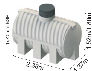
HZ03000 (AG/UG) (3,044 ltrs)
